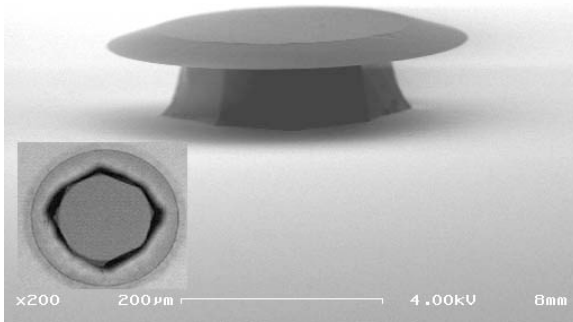
Figure 1: SEM image of 400 μm disk; inset: top down view taken with optical microscope.
