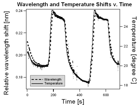
Figure 3: Changes in Wavelength and Temperature v. Time.
